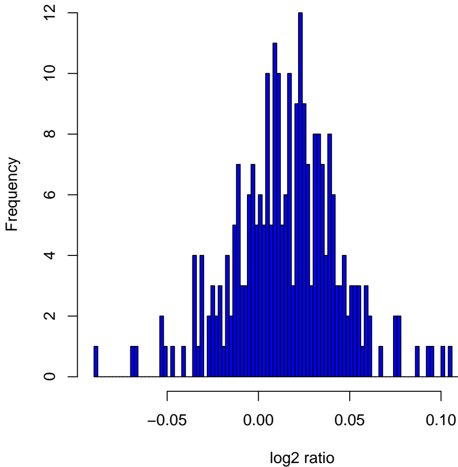
Histogram of log 2 ratios in 270 HapMap samples at clone Chr7tp-20F6
