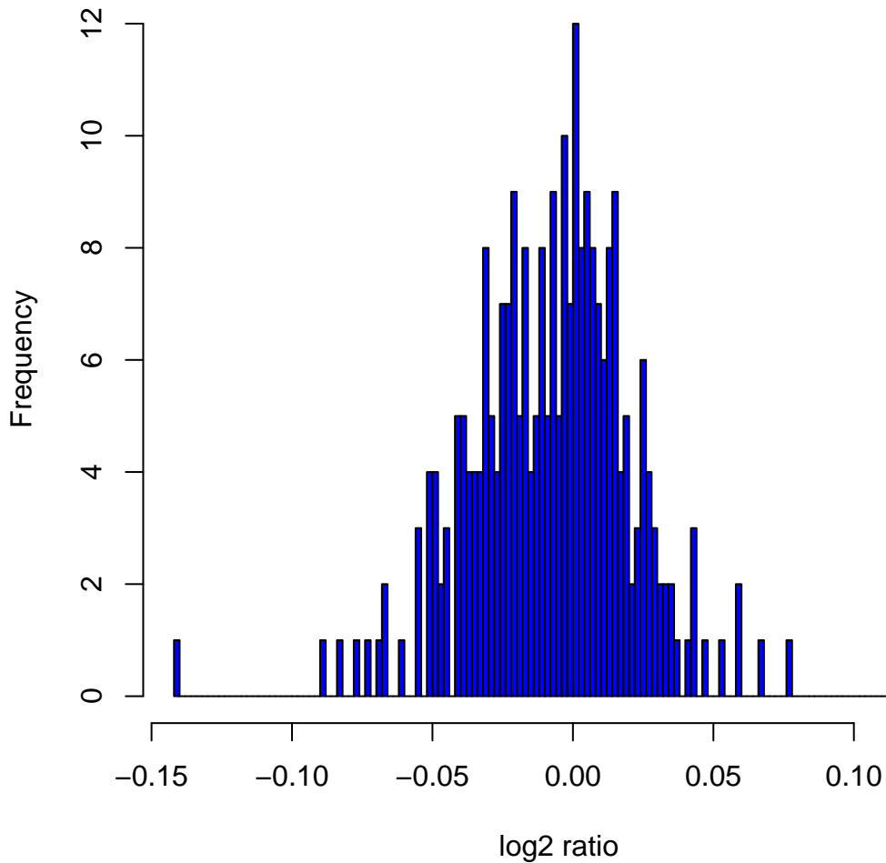
Histogram of log 2 ratios in 270 HapMap samples at clone Chr7tp-20G2
