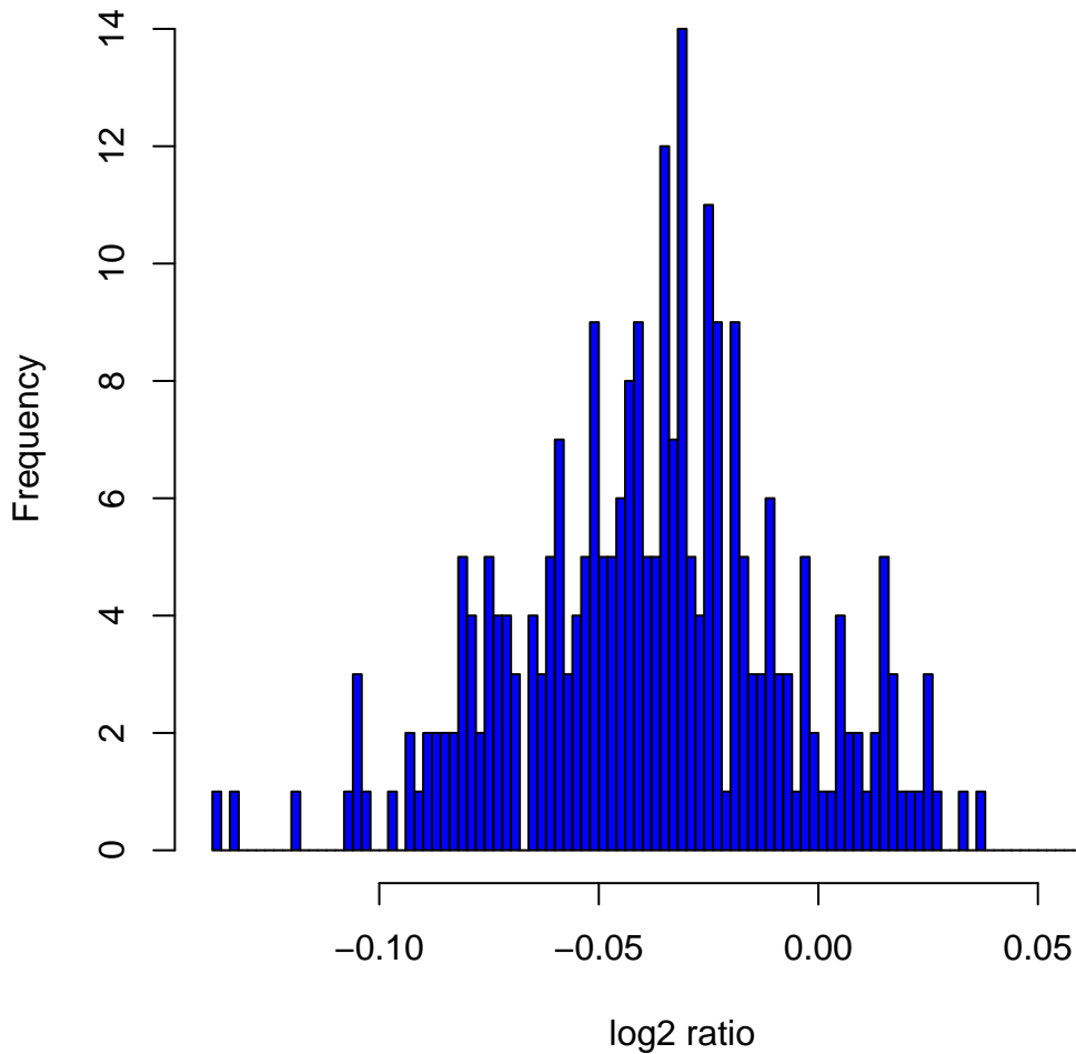
Histogram of log 2 ratios in 270 HapMap samples at clone Chr7tp-20G6
