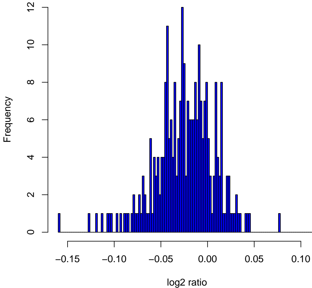
Histogram of log 2 ratios in 270 HapMap samples at clone Chr7tp-20G7
