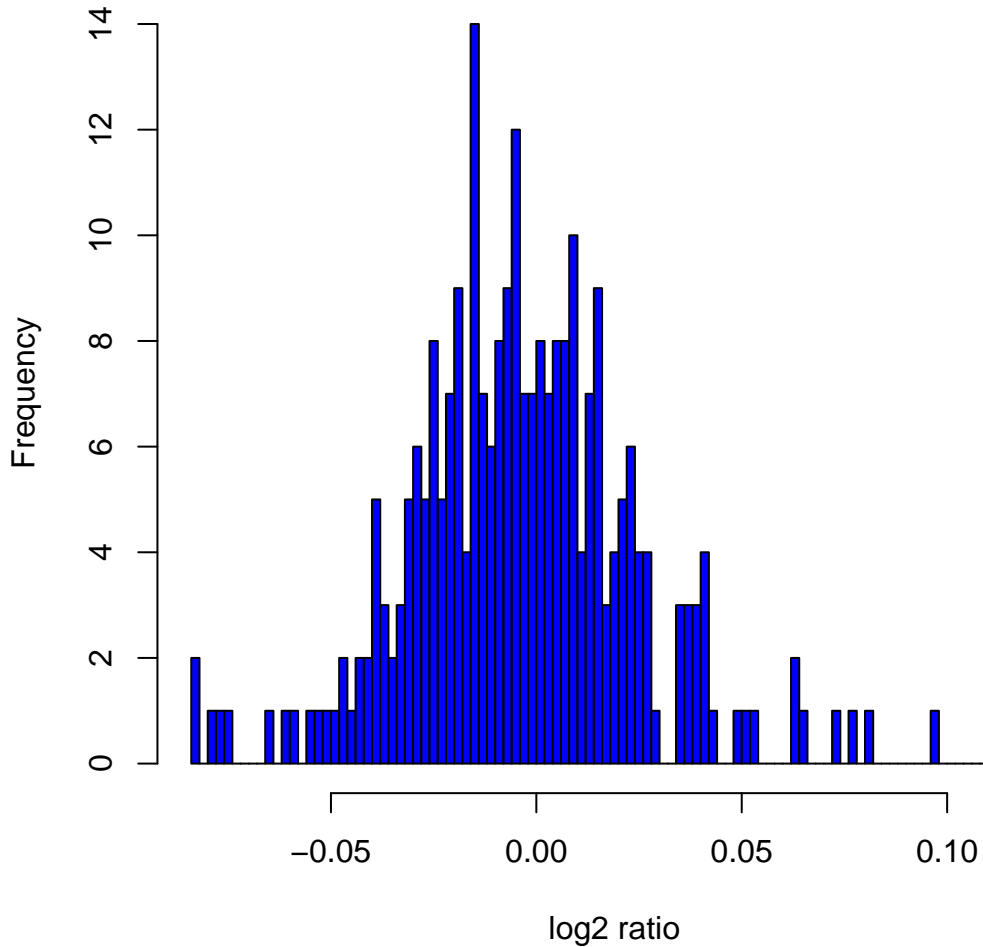
Histogram of log 2 ratios in 270 HapMap samples at clone Chr7tp-21A2
