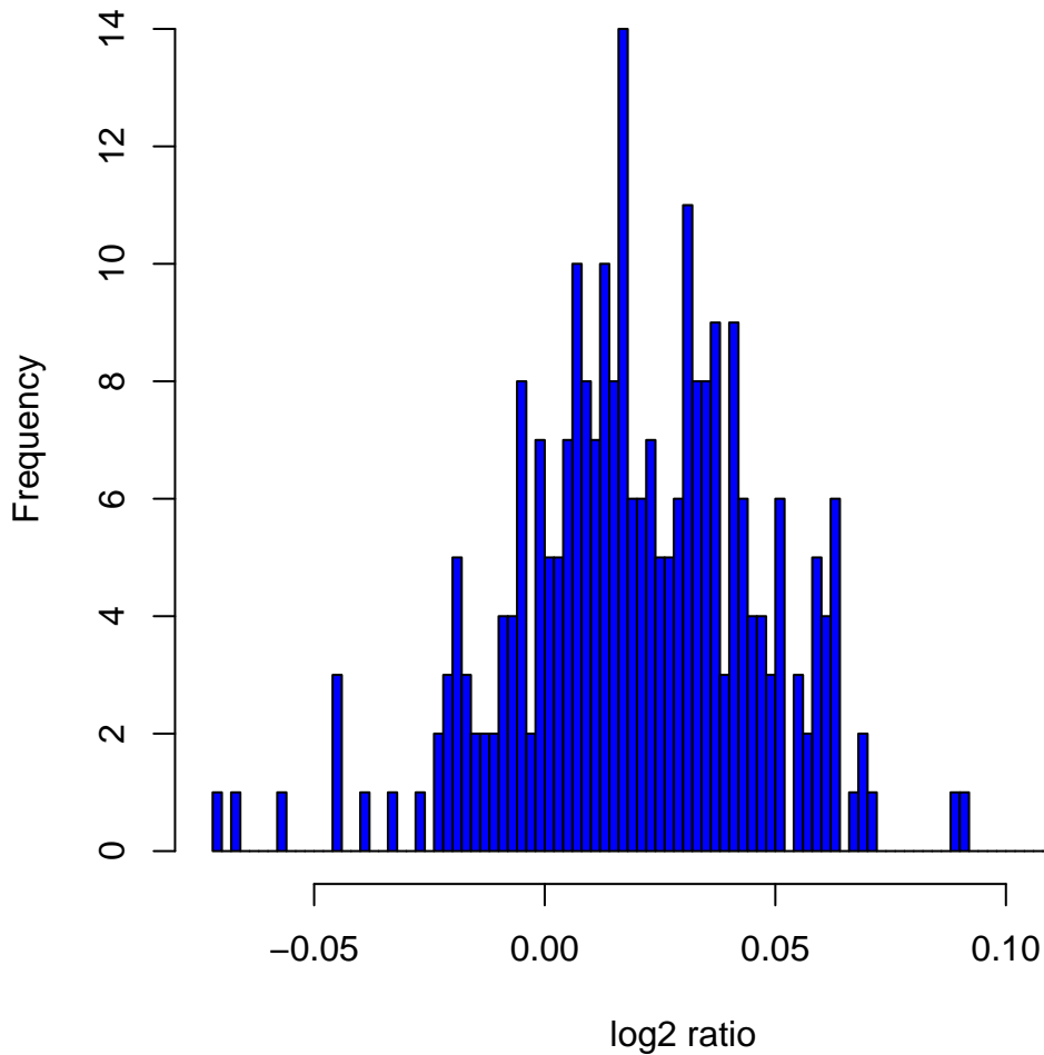
Histogram of log 2 ratios in 270 HapMap samples at clone Chr7tp-21B2
