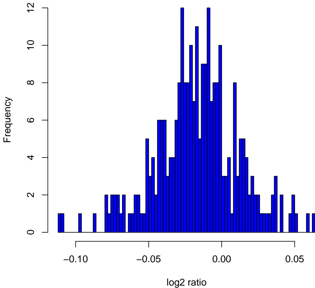
Histogram of log 2 ratios in 270 HapMap samples at clone Chr7tp-21B6
