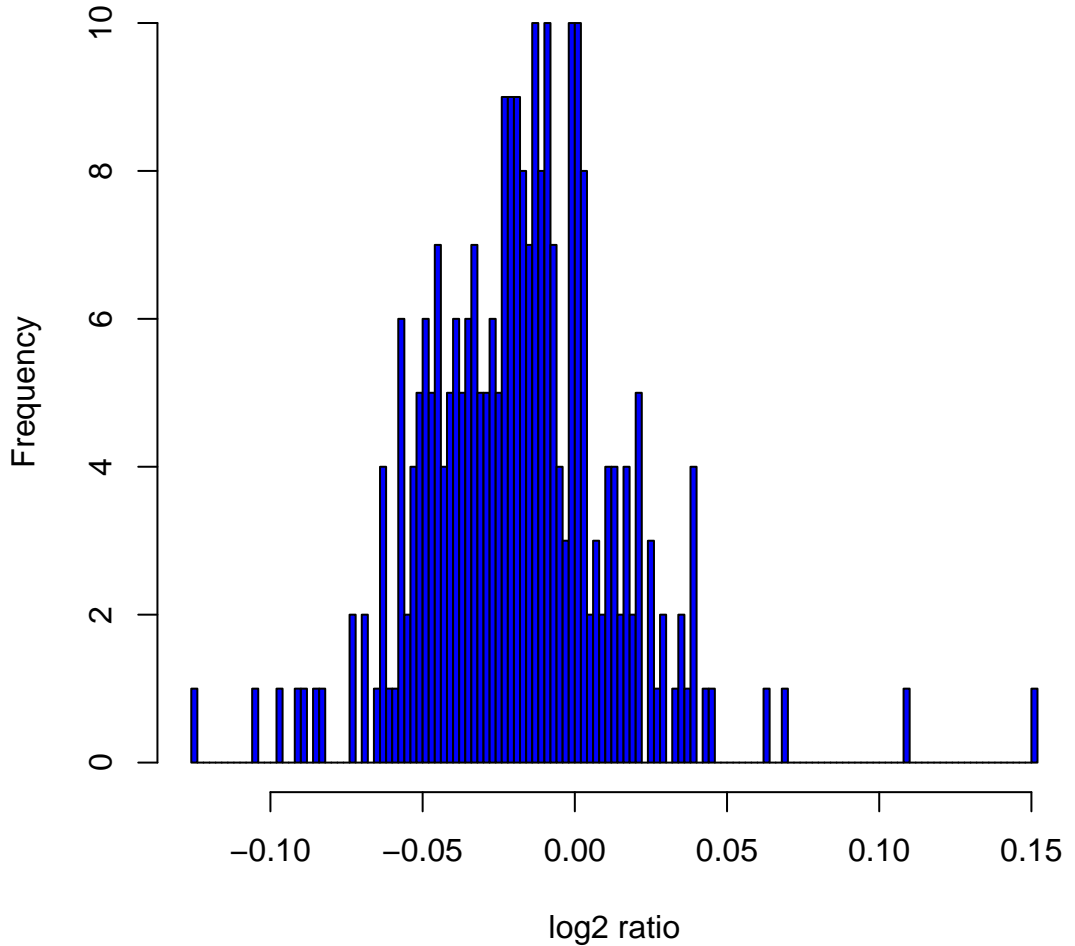
Histogram of log 2 ratios in 270 HapMap samples at clone Chr7tp-21D6
