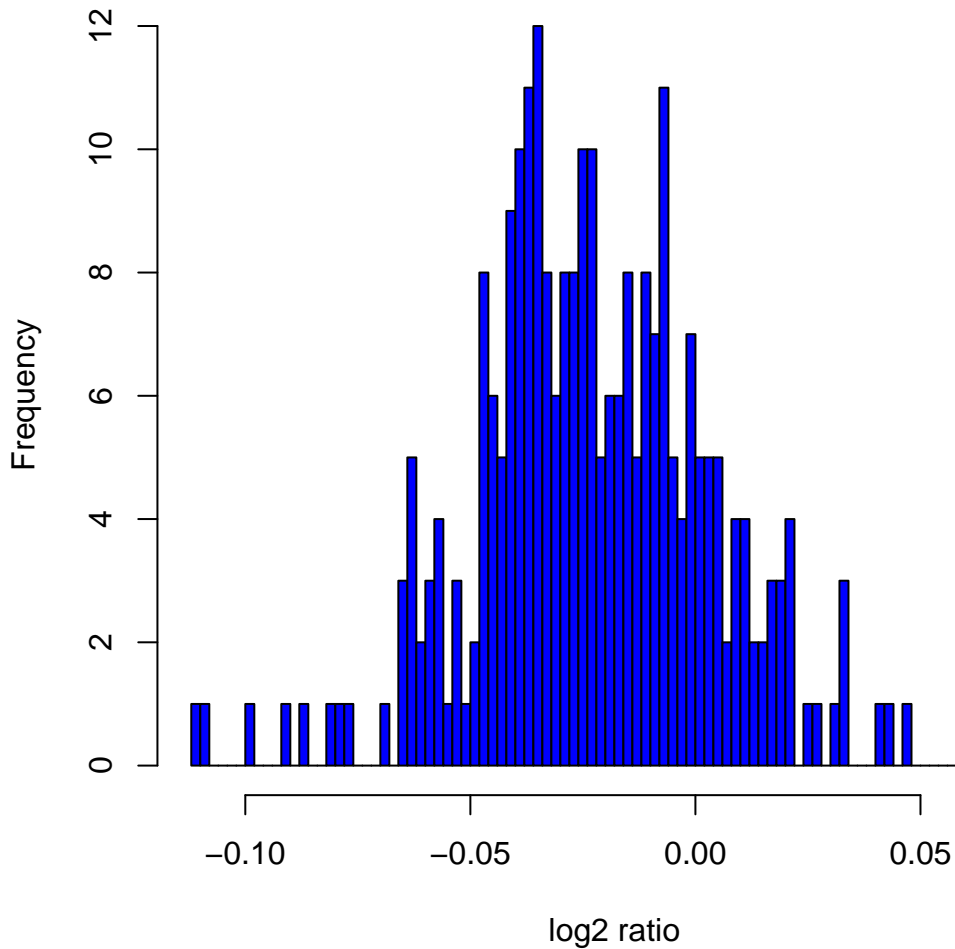
Histogram of log2ratios in 270 HapMap samples at clone Chr7tp-21E11
