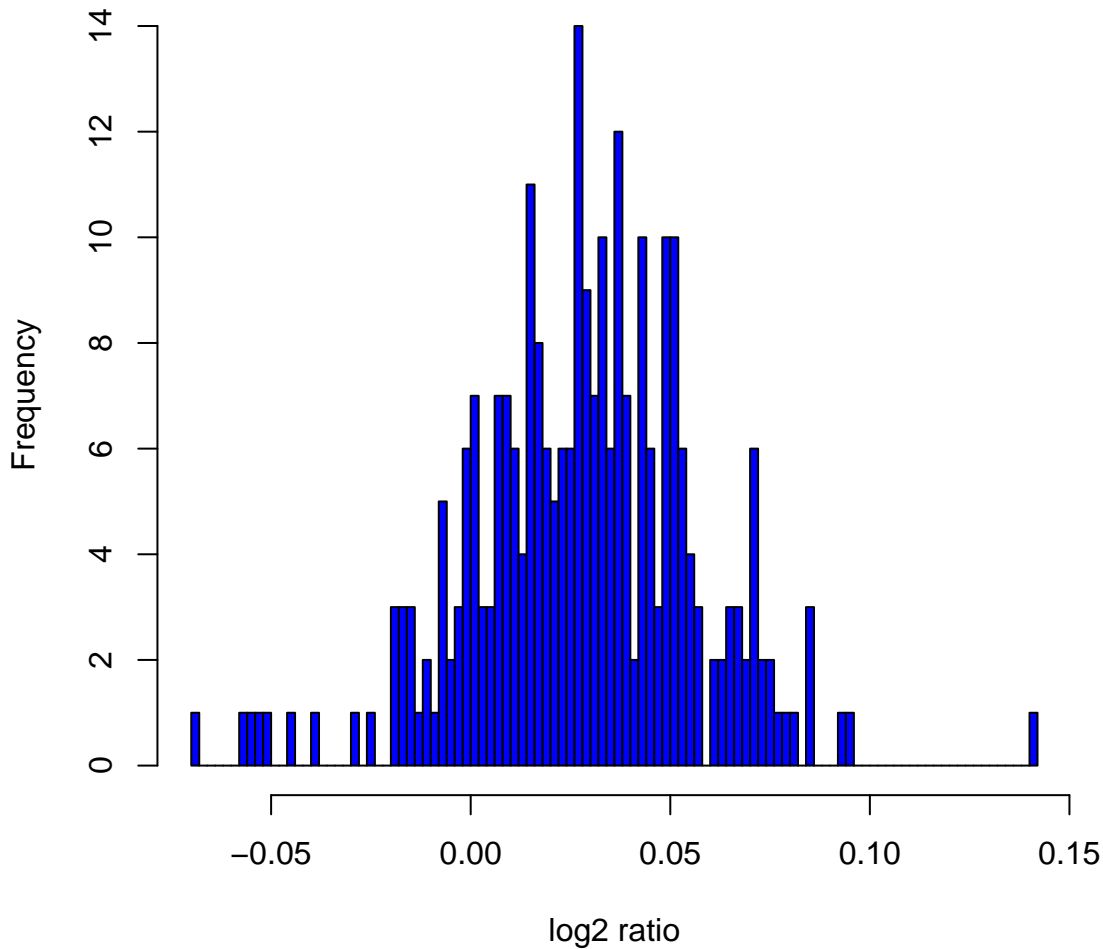
Histogram of log 2 ratios in 270 HapMap samples at clone Chr7tp-21E2
