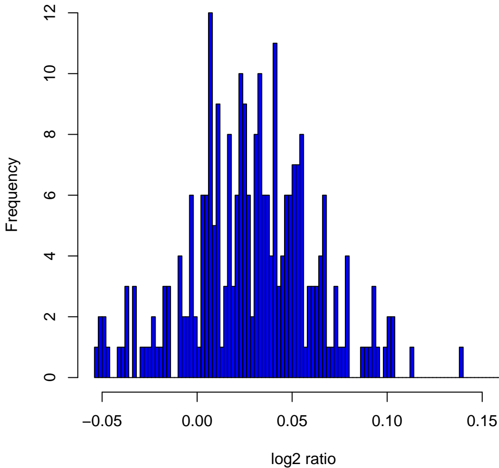
Histogram of log2ratios in 270 HapMap samples at clone Chr7tp-21F11
