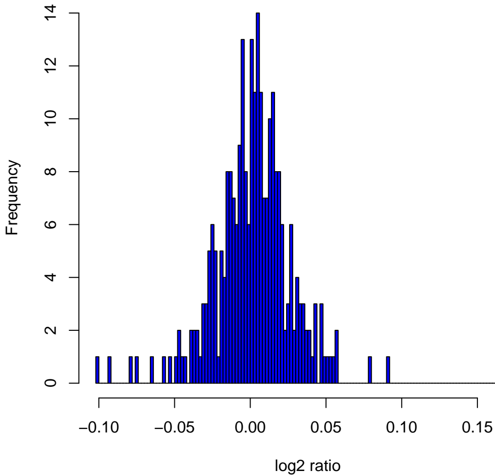
Histogram of \log_2 ratios in 270 HapMap samples at clone Chr7tp-21G2
