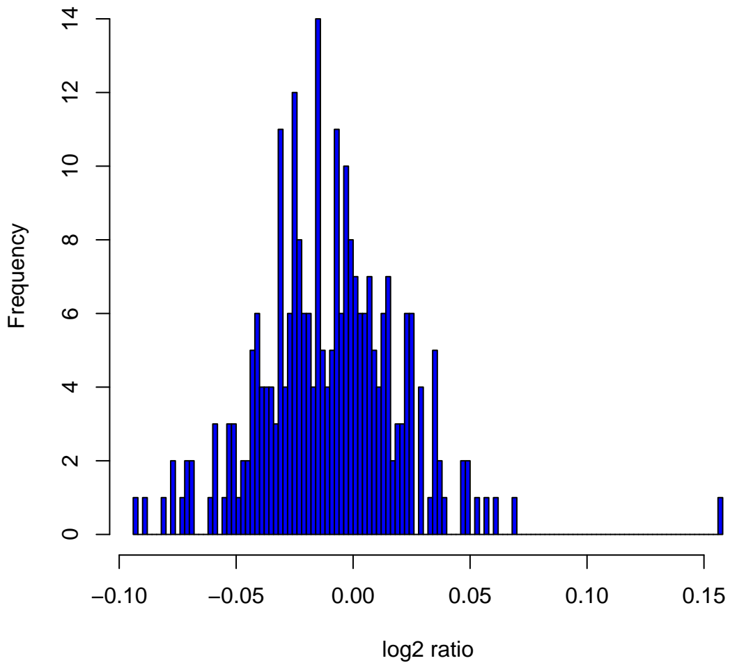
Histogram of log 2 ratios in 270 HapMap samples at clone Chr7tp-21H8
