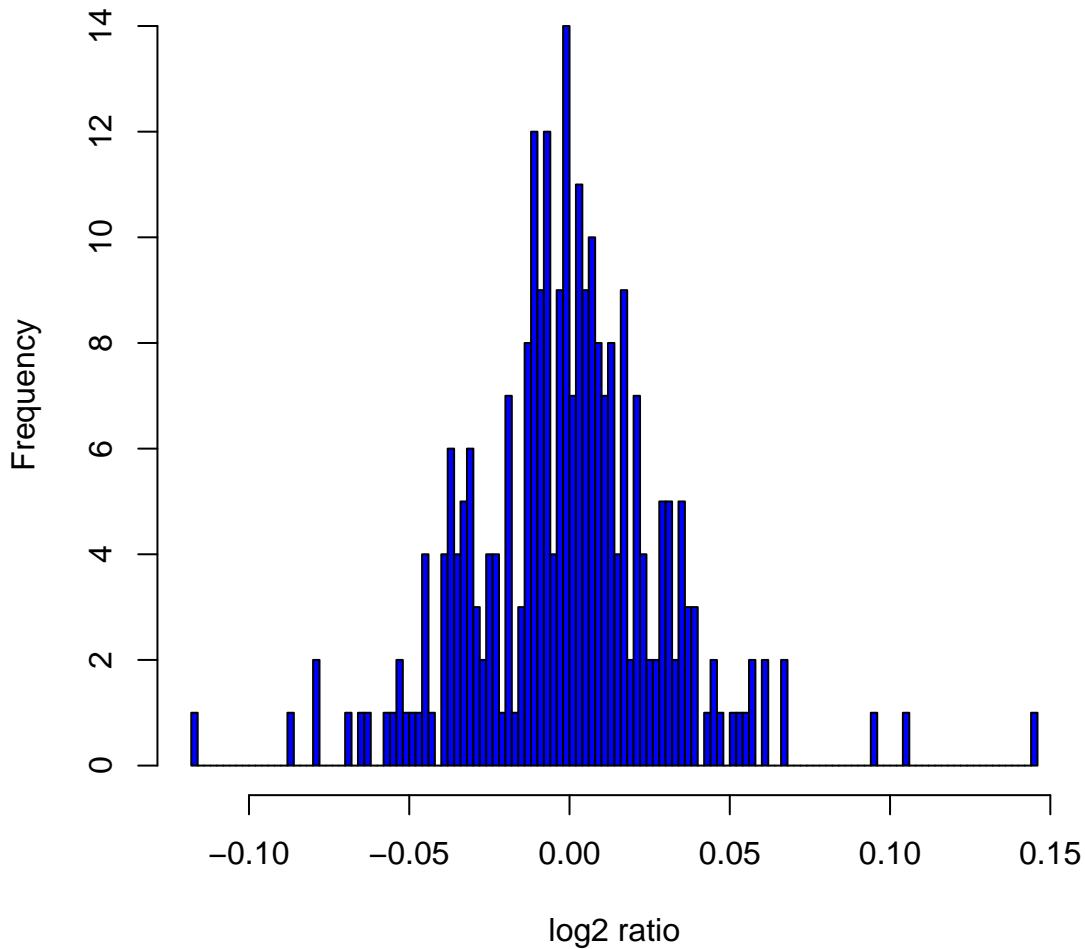
Histogram of log2ratios in 270 HapMap samples at clone Chr7tp-23A10
