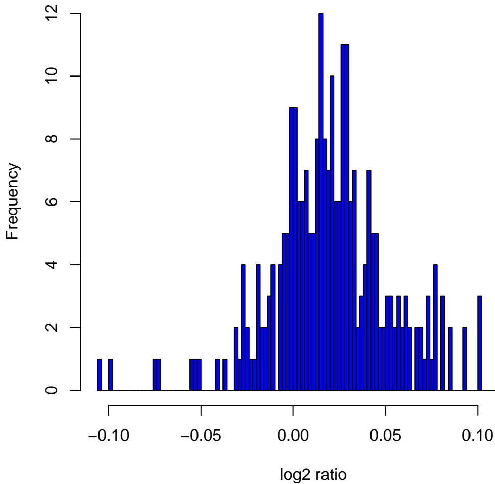
Histogram of log 2 ratios in 270 HapMap samples at clone Chr7tp-23B4
