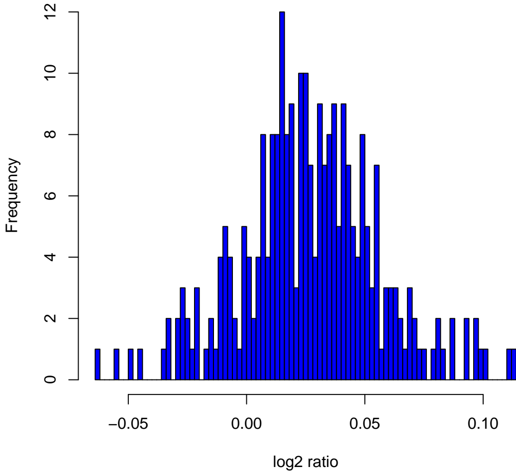
Histogram of \log_2 ratios in 270 HapMap samples at clone Chr7tp-23G2
