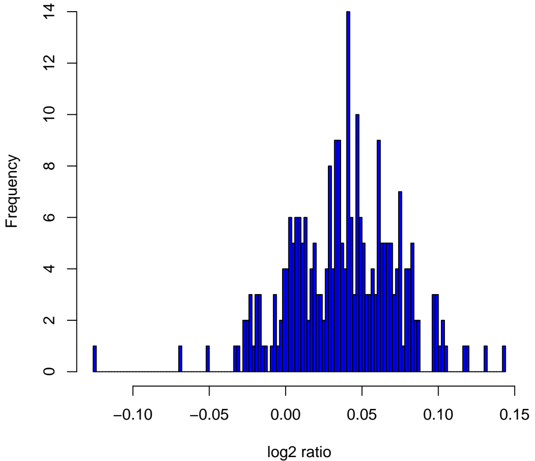
Histogram of log2ratios in 270 HapMap samples at clone Chr7tp-23G6
