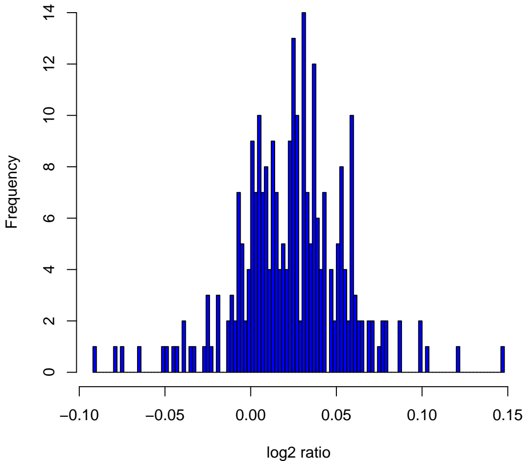
Histogram of log 2 ratios in 270 HapMap samples at clone Chr7tp-24A5
