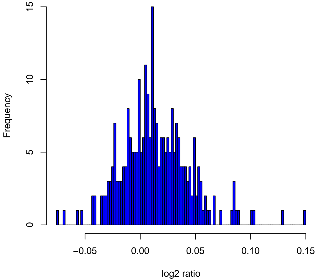
Histogram of log 2 ratios in 270 HapMap samples at clone Chr7tp-24C2
