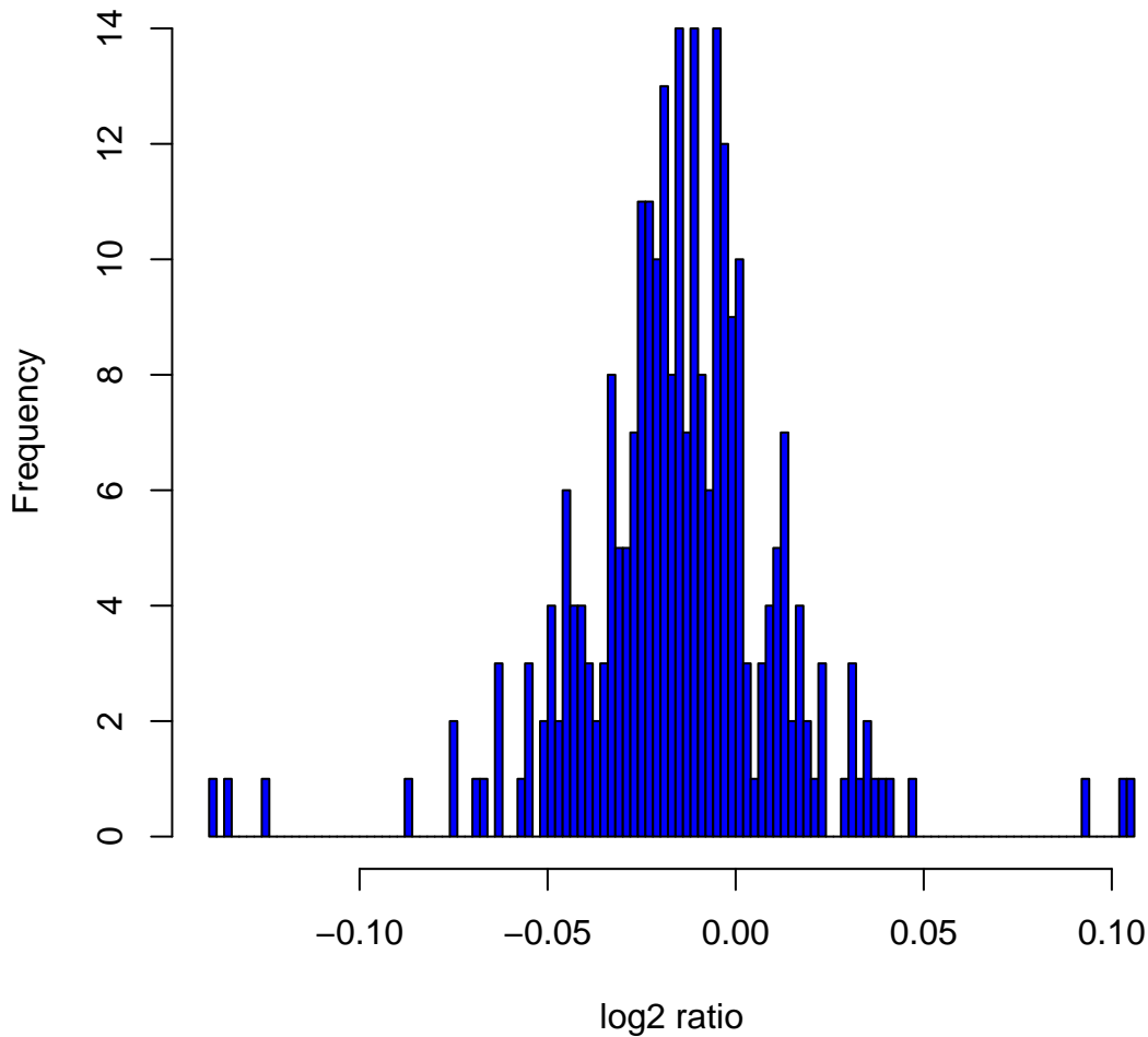
Histogram of log 2 ratios in 270 HapMap samples at clone Chr7tp-2E1
