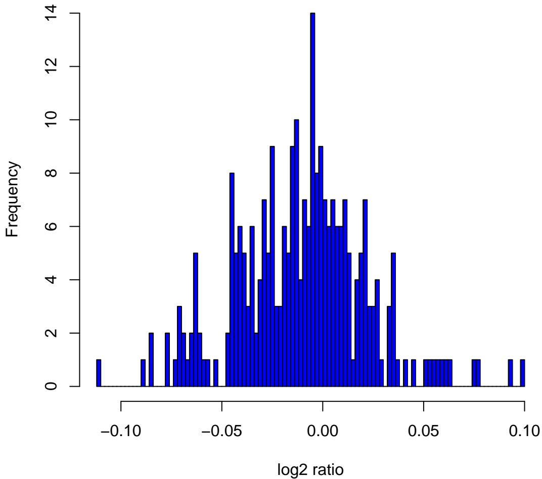
Histogram of \log_2 ratios in 270 HapMap samples at clone Chr7tp-2H4
