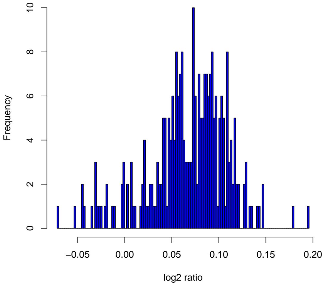
Histogram of log 2 ratios in 270 HapMap samples at clone Chr7tp-3A5
