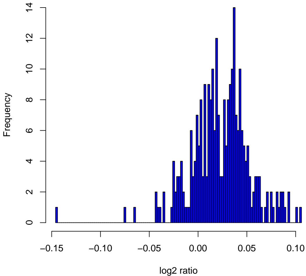
Histogram of log 2 ratios in 270 HapMap samples at clone Chr7tp-3A8
