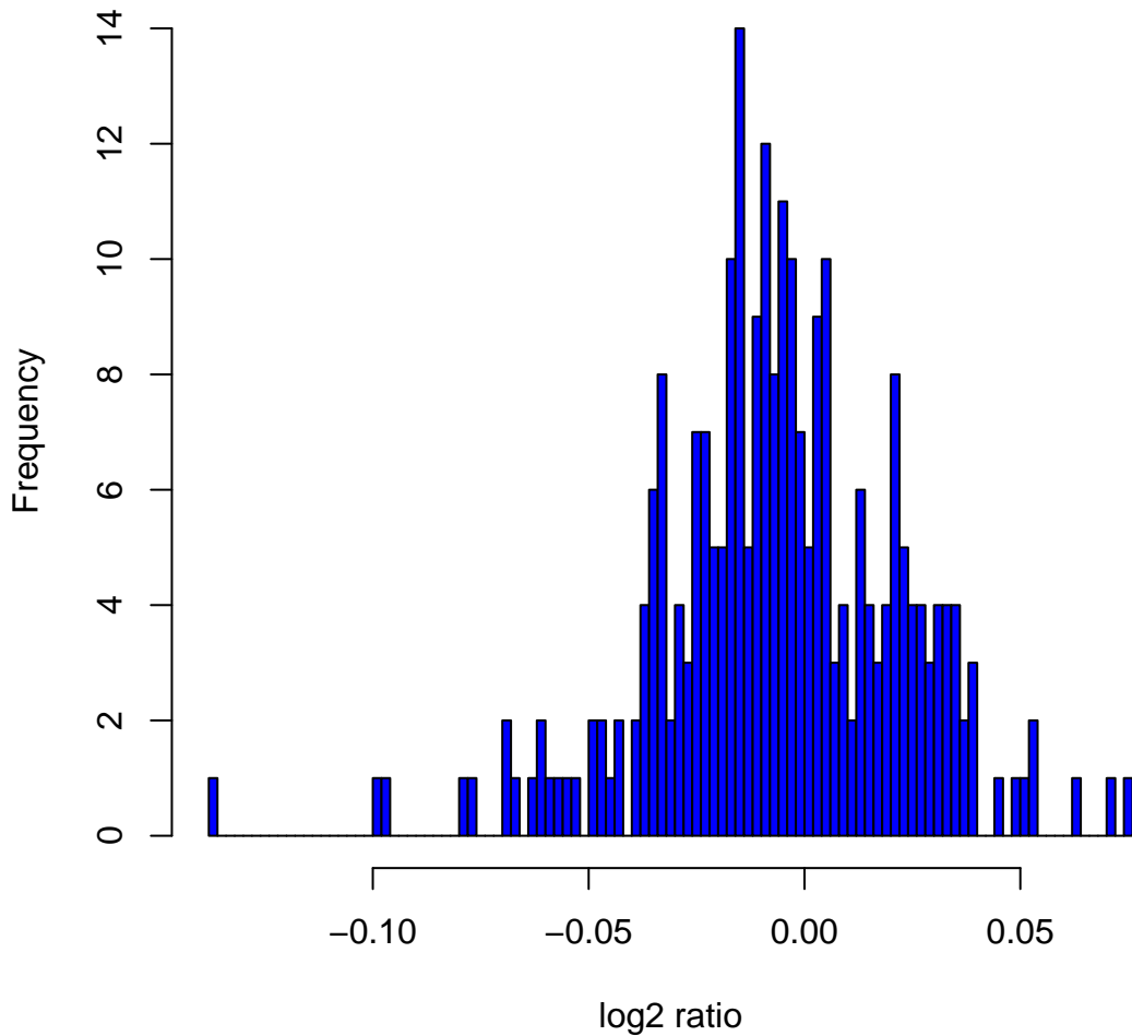
Histogram of log 2 ratios in 270 HapMap samples at clone Chr7tp-3B9
