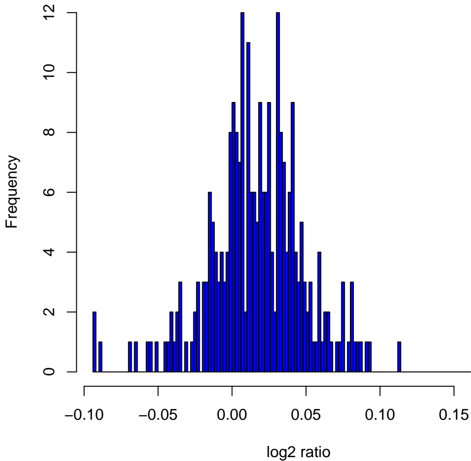
Histogram of log 2 ratios in 270 HapMap samples at clone Chr7tp-3C5
