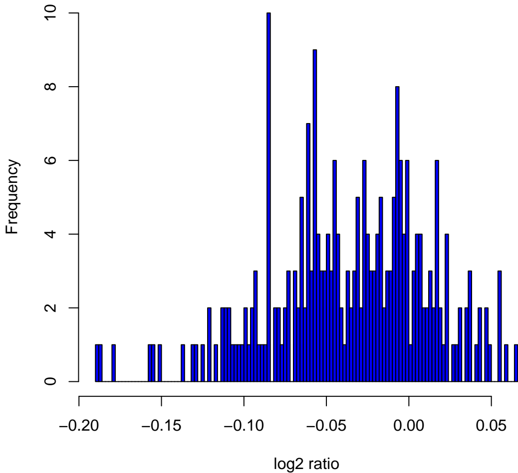
Histogram of log 2 ratios in 270 HapMap samples at clone Chr7tp-3D6
