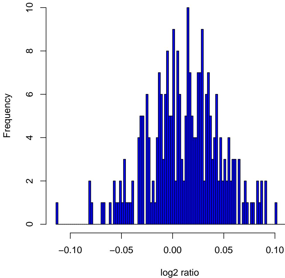
Histogram of \log_2 ratios in 270 HapMap samples at clone Chr7tp-3D7
