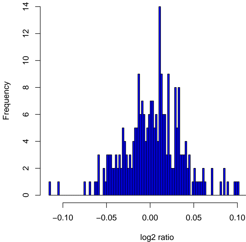
Histogram of log 2 ratios in 270 HapMap samples at clone Chr7tp-3E1
