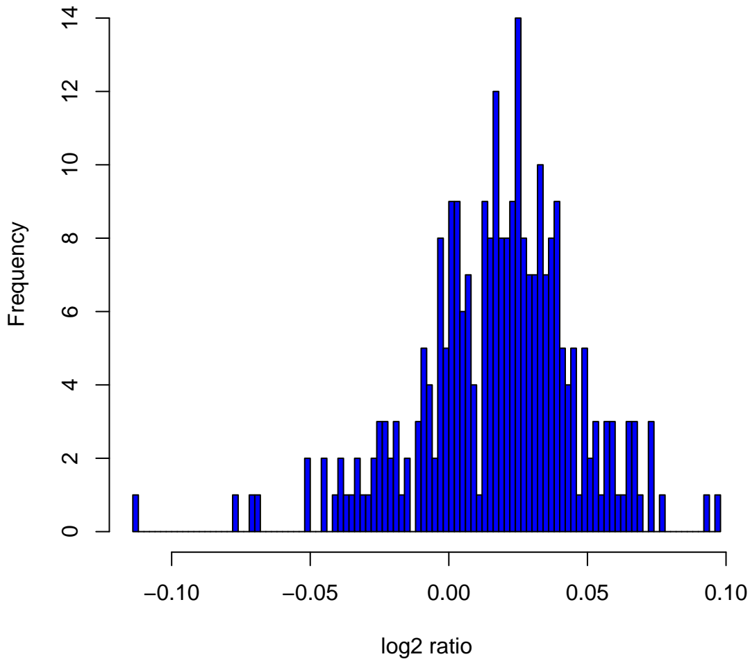
Histogram of log2ratios in 270 HapMap samples at clone Chr7tp-3E5
