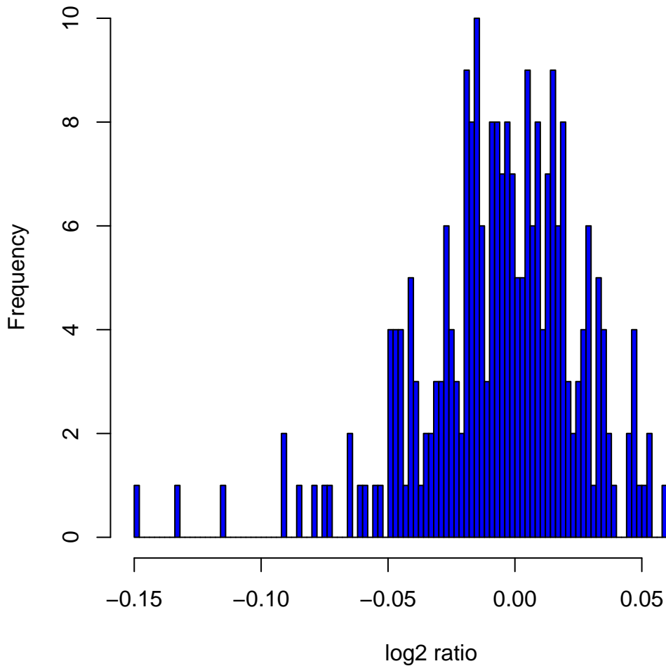
Histogram of log2ratios in 270 HapMap samples at clone Chr7tp-3F1
