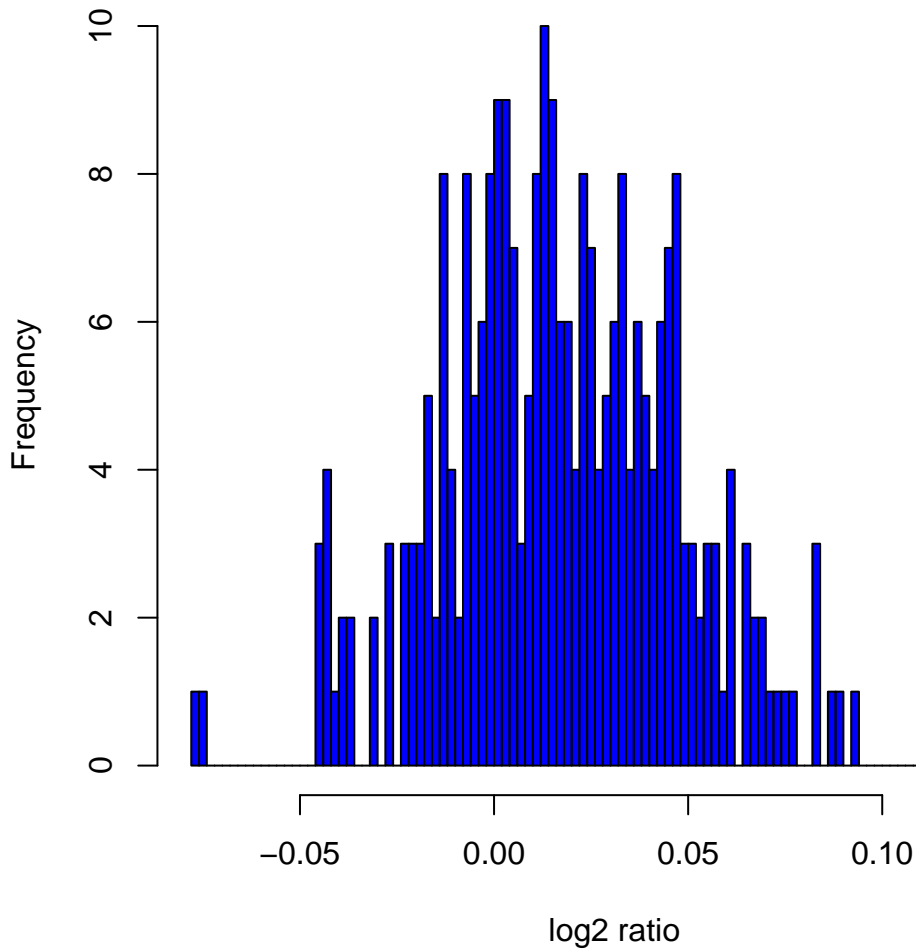
Histogram of \log_2 ratios in 270 HapMap samples at clone Chr7tp-3F12
