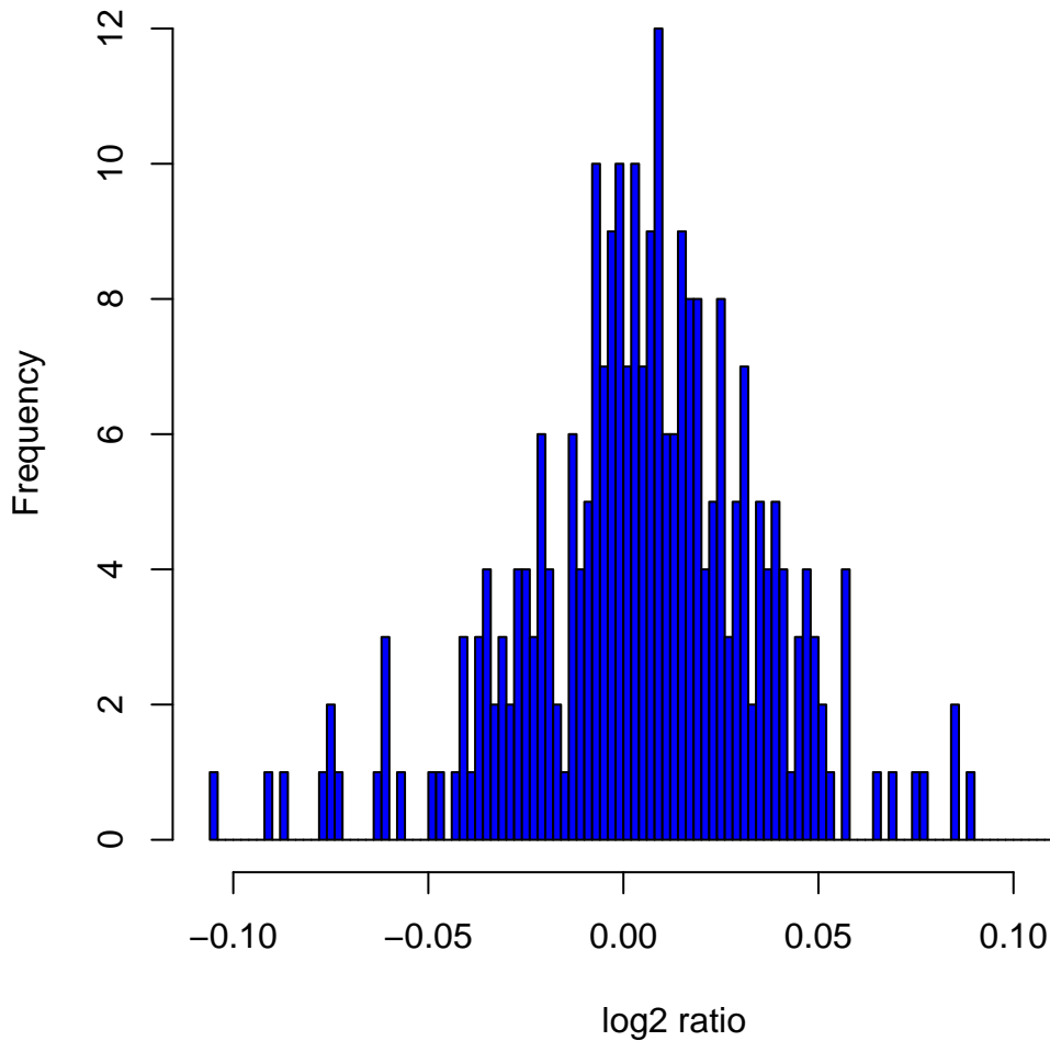
Histogram of log2ratios in 270 HapMap samples at clone Chr7tp-3G1
