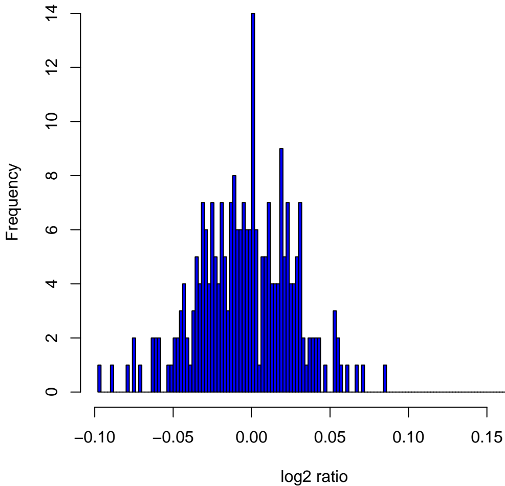
Histogram of \log_2 ratios in 270 HapMap samples at clone Chr7tp-3H5
