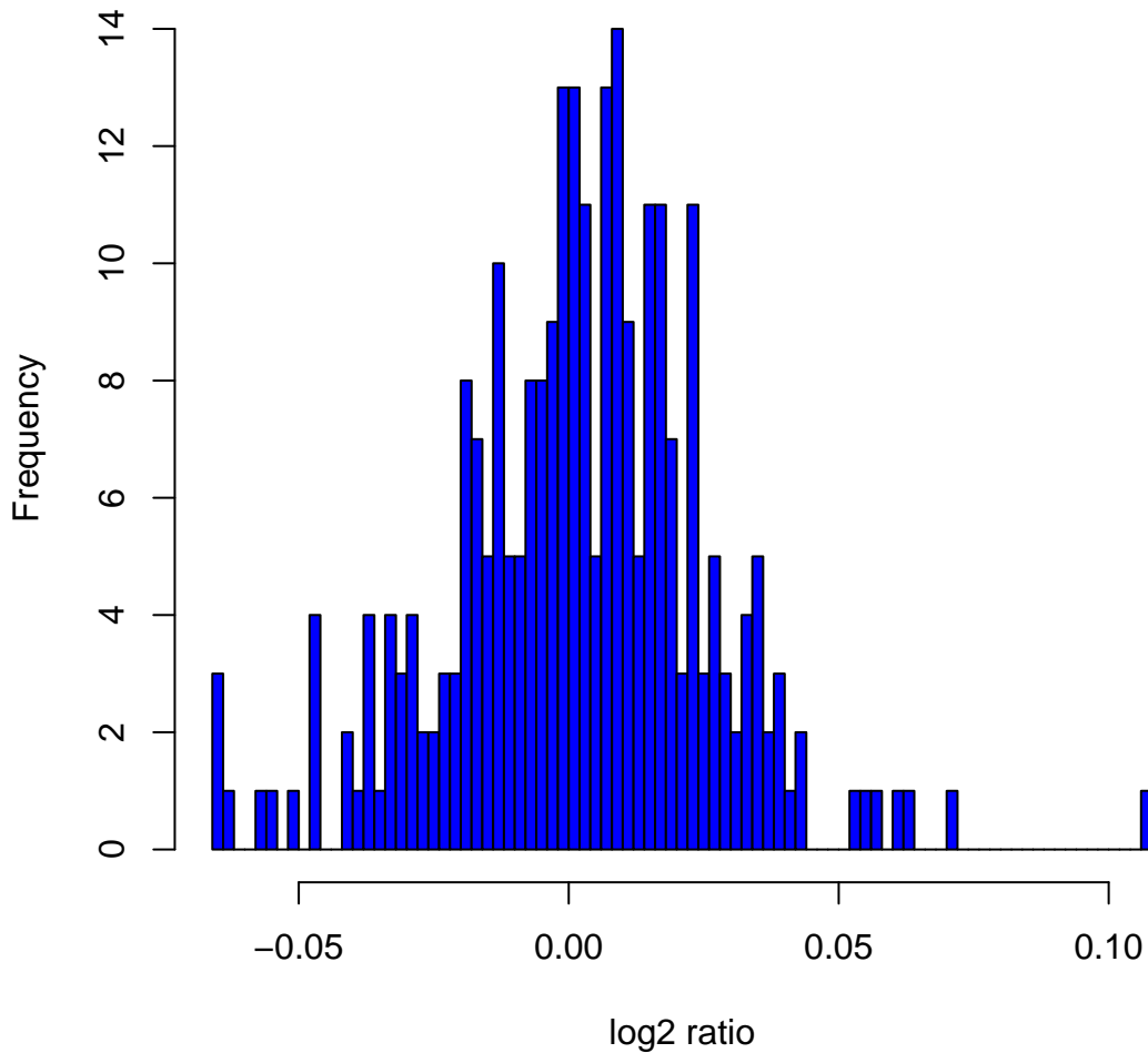
Histogram of log 2 ratios in 270 HapMap samples at clone Chr7tp-4A4
