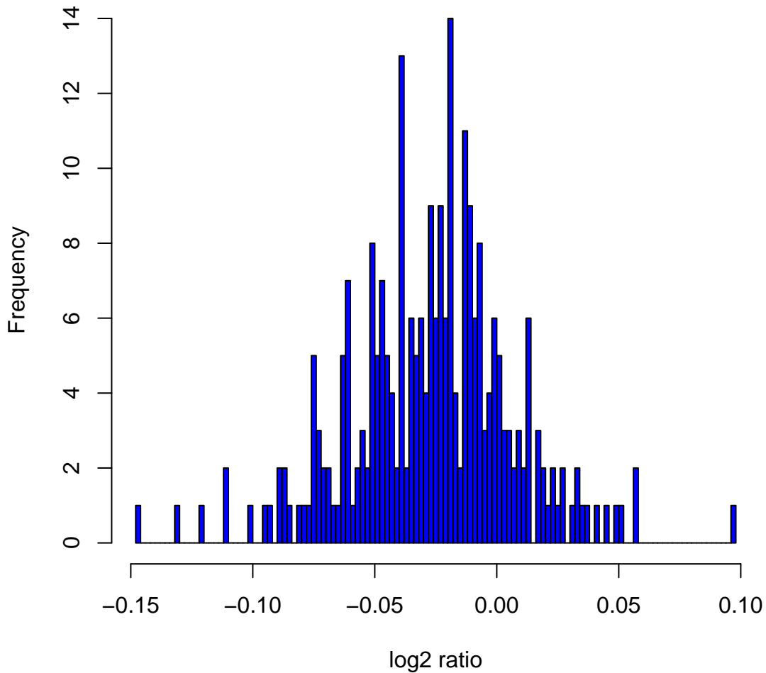
Histogram of log2ratios in 270 HapMap samples at clone Chr7tp-4A5
