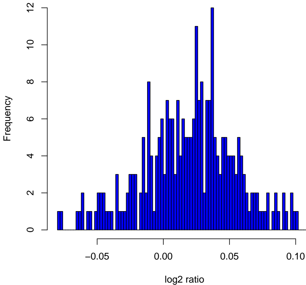
Histogram of \log_2 ratios in 270 HapMap samples at clone Chr7tp-4C6
