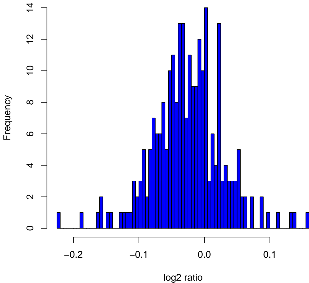
Histogram of \log_2 ratios in 270 HapMap samples at clone Chr7tp-4D8
