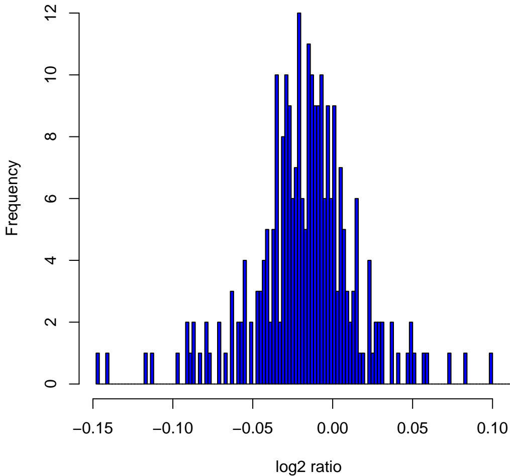
Histogram of log 2 ratios in 270 HapMap samples at clone Chr7tp-4D9
