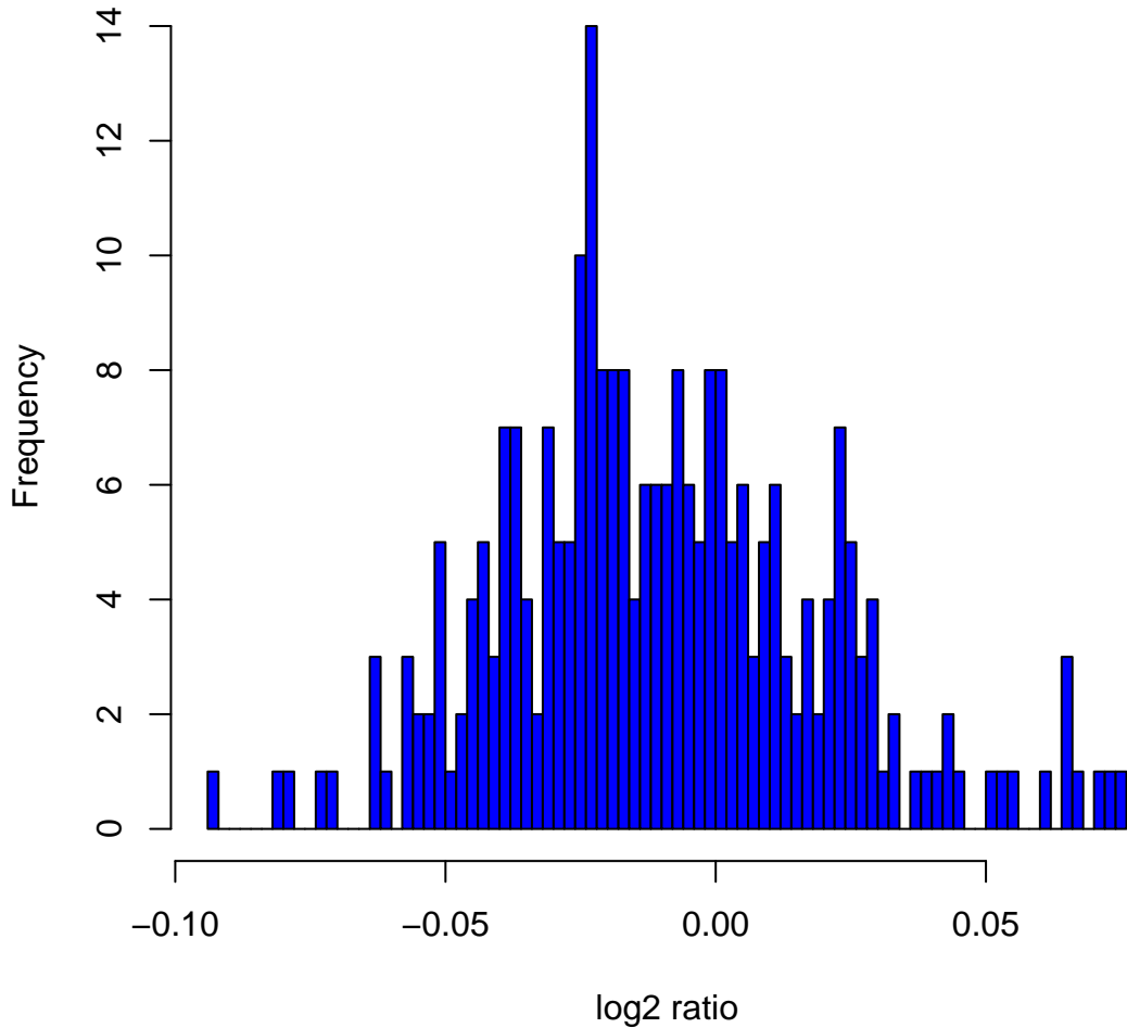
Histogram of log 2 ratios in 270 HapMap samples at clone Chr7tp-4F3
