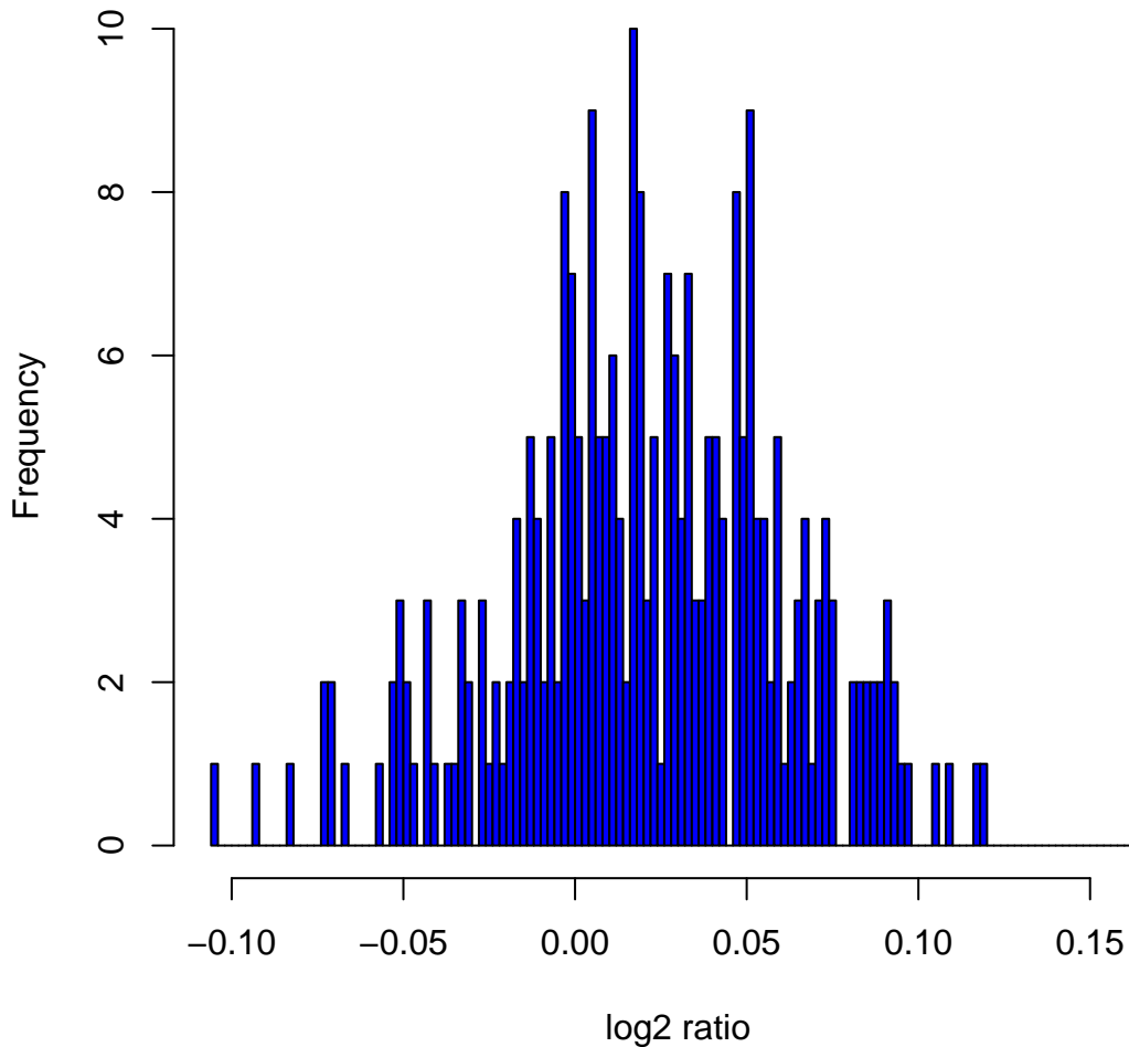
Histogram of log 2 ratios in 270 HapMap samples at clone Chr7tp-4G9
