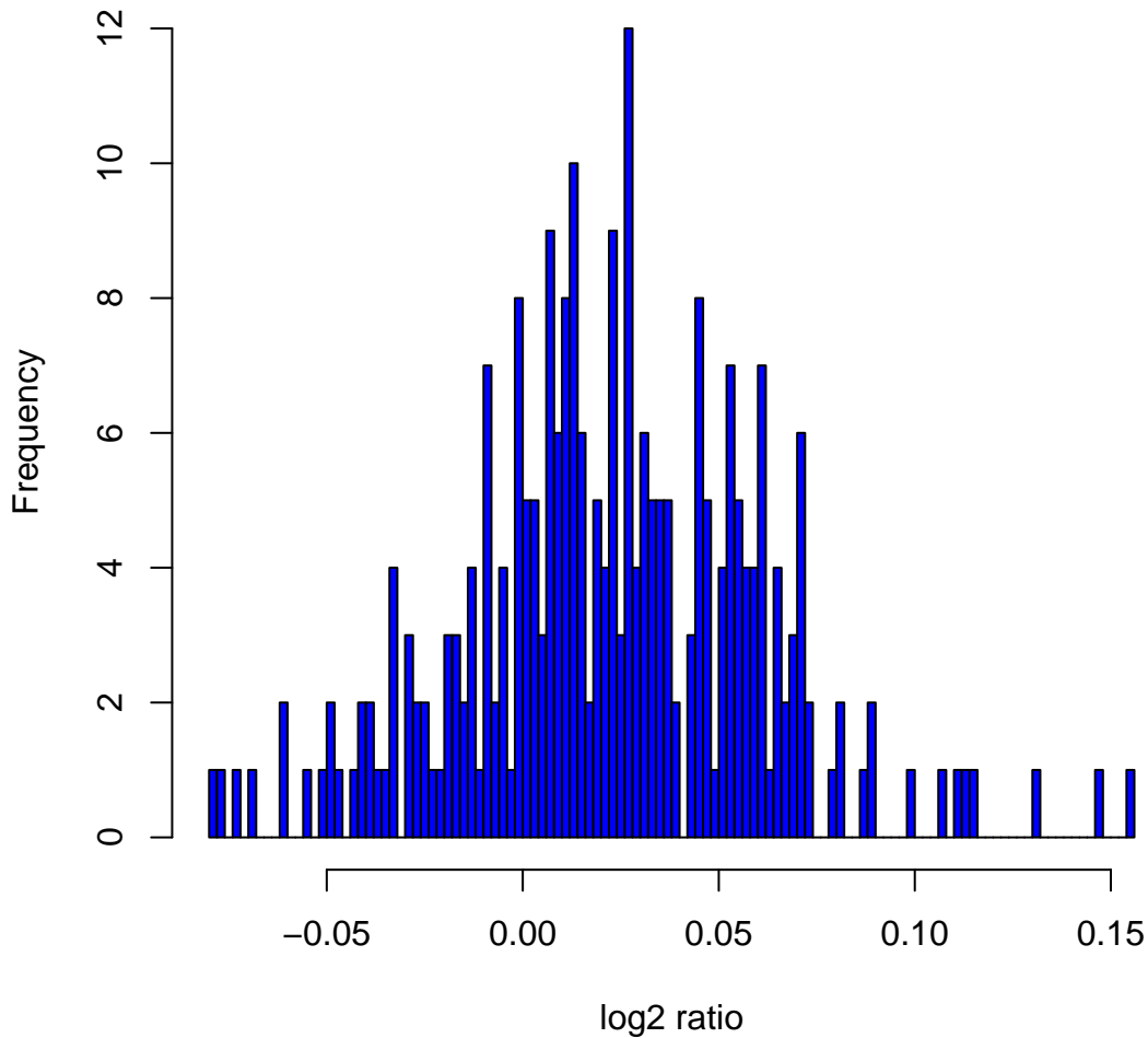
Histogram of log 2 ratios in 270 HapMap samples at clone Chr7tp-4H3
