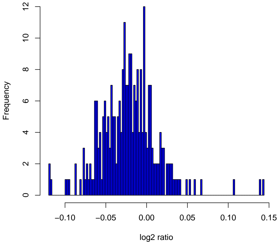
Histogram of log 2 ratios in 270 HapMap samples at clone Chr7tp-4H8
