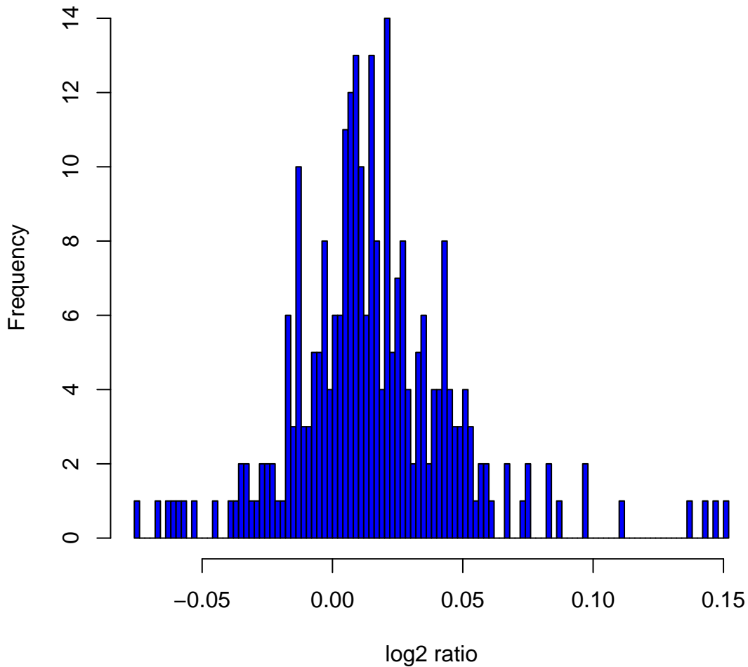
Histogram of log 2 ratios in 270 HapMap samples at clone Chr7tp-5A3
