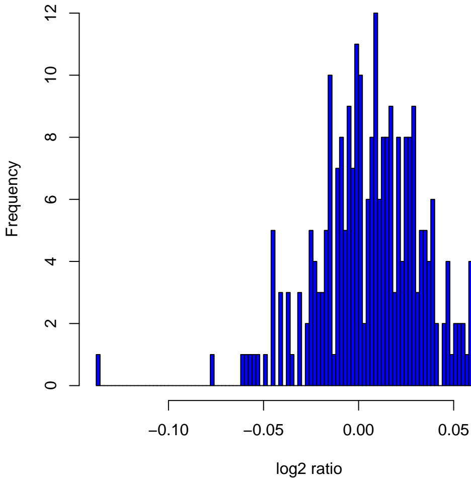
Histogram of \log_2 ratios in 270 HapMap samples at clone Chr7tp-5A5
