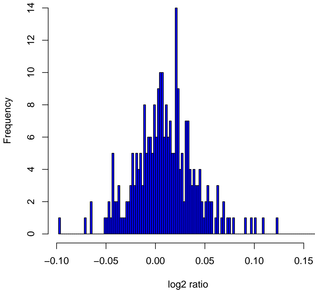
Histogram of log 2 ratios in 270 HapMap samples at clone Chr7tp-5A7
