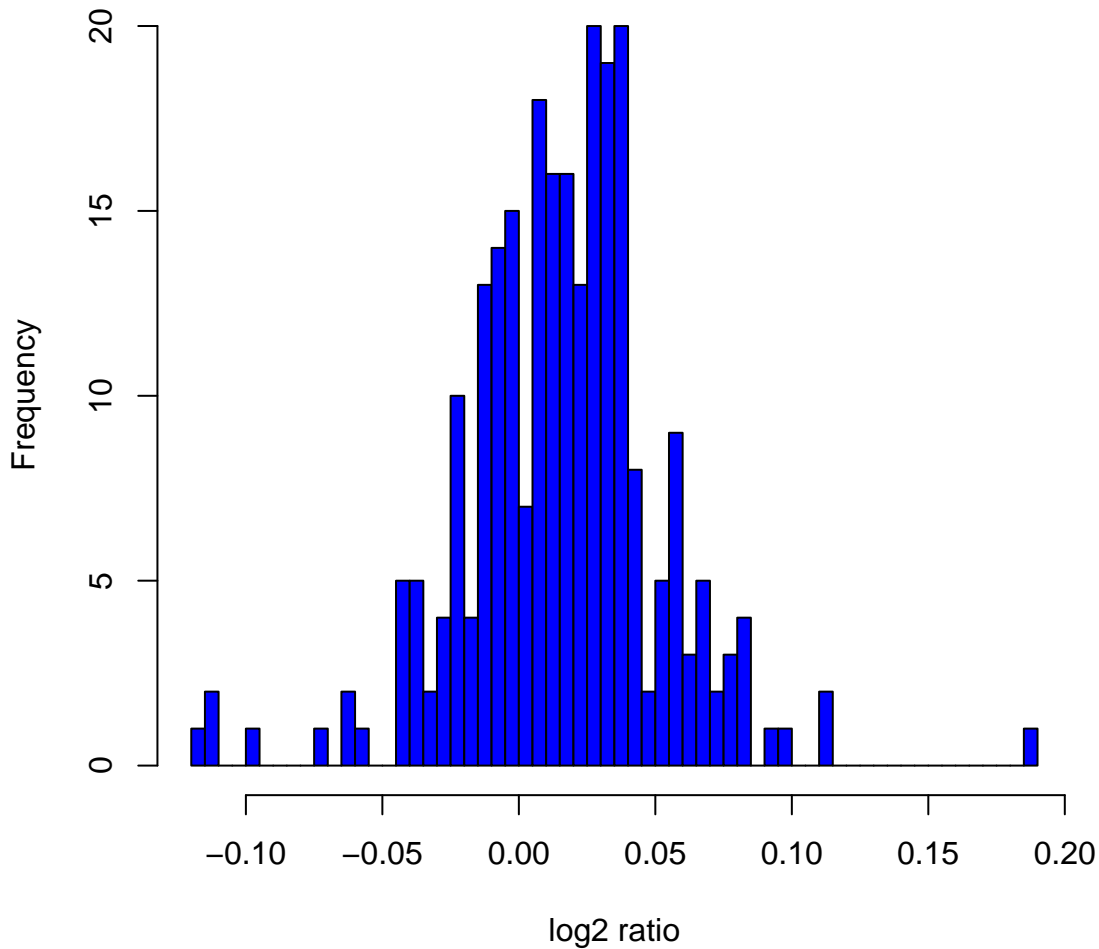
Histogram of log 2 ratios in 270 HapMap samples at clone Chr7tp-5D5
