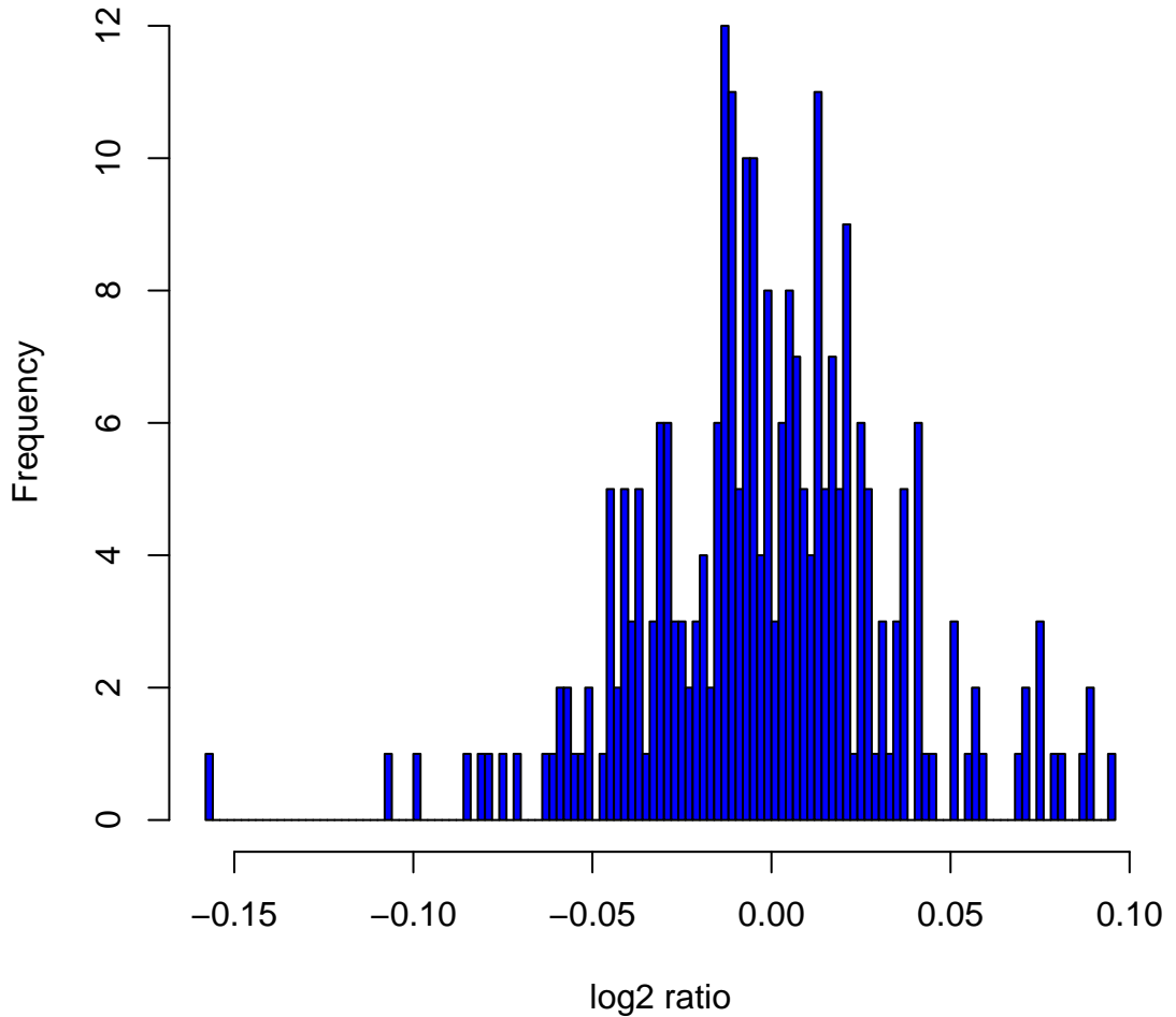
Histogram of log 2 ratios in 270 HapMap samples at clone Chr7tp-5F9
