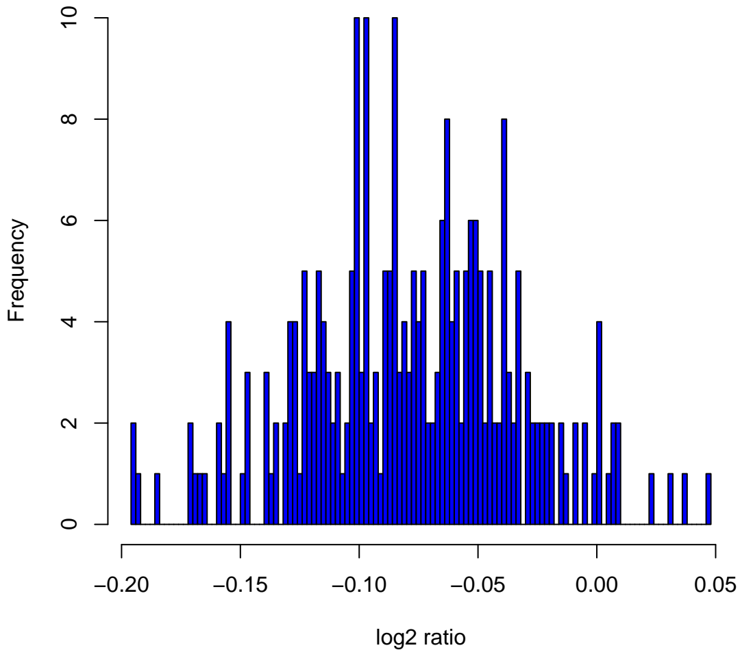
Histogram of log2ratios in 270 HapMap samples at clone Chr7tp-5G10
