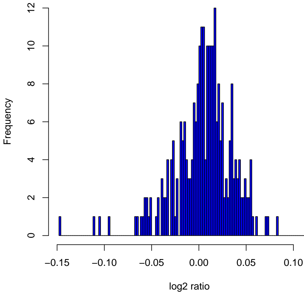
Histogram of log 2 ratios in 270 HapMap samples at clone Chr7tp-5G3
