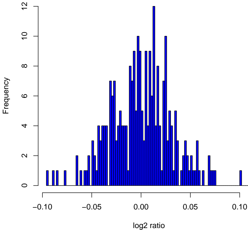
Histogram of log2ratios in 270 HapMap samples at clone Chr7tp-5H1
